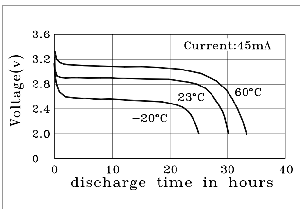
Discharge characteristics vs. temperature
